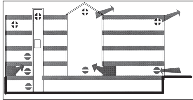
Figure 2: Stack effect.
