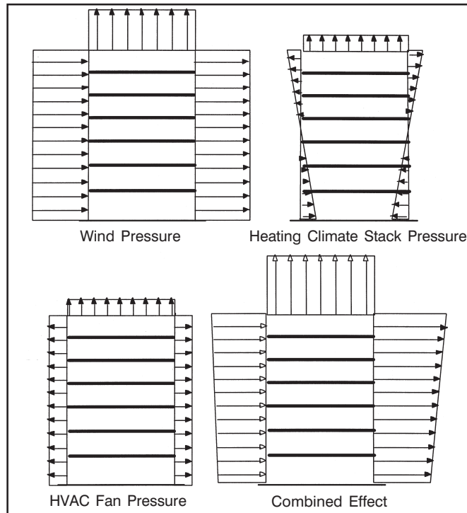
Figure 3: Combined wind, stack and fan pressure.
